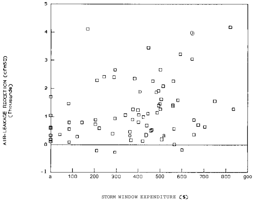
Fig. 5.5. Comparison of air-leakage reduction for each house following weatherization to the expenditure for storm windows in the house.
